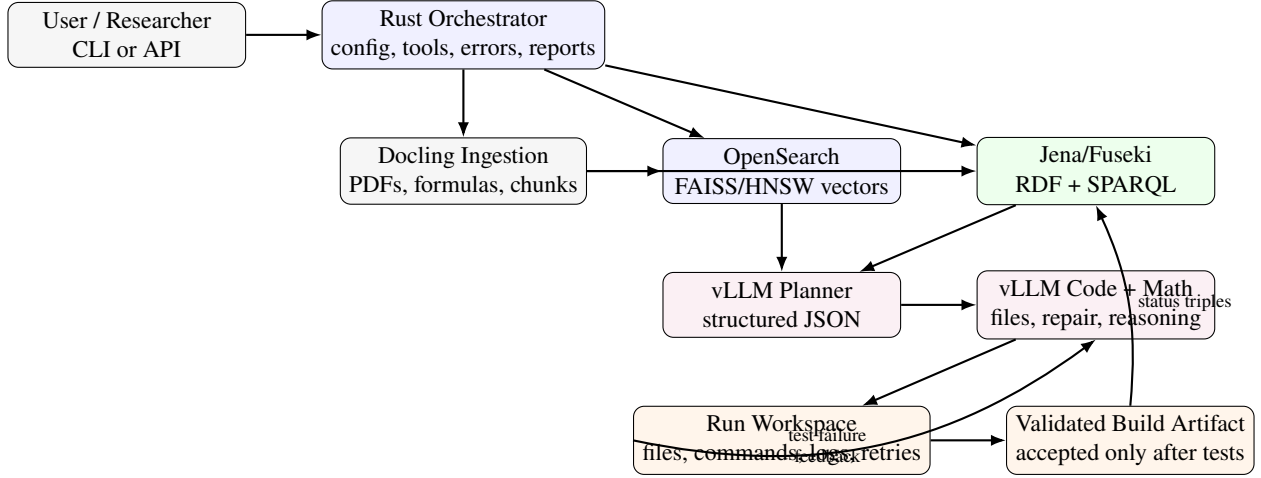
Figure 1: VERITAS reference architecture. Retrieval gives similarity; RDF/SPARQL gives semantic roles; vLLM gives model planning and generation; the run workspace gives auditable execution.
