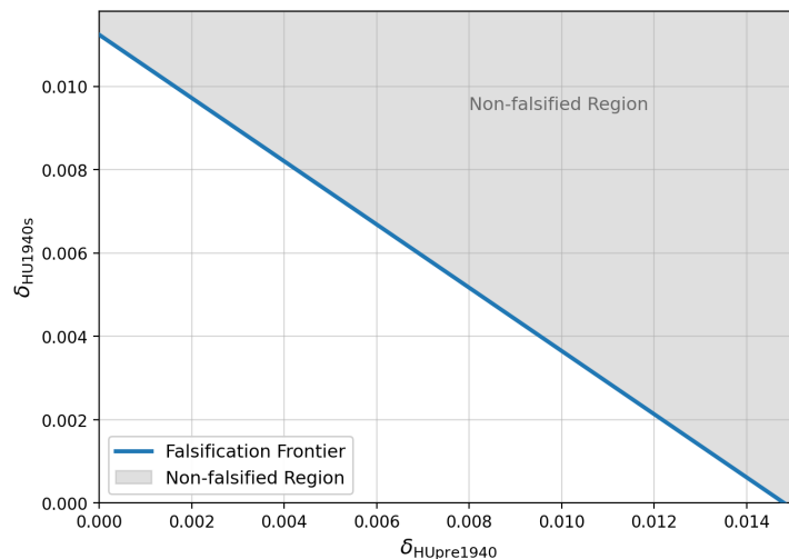
Figure 1: Estimated falsification frontier
