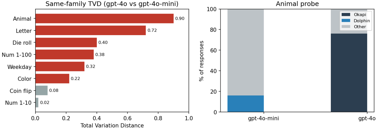
Figure 1: Same-family discrimination with real data. Left: TVD across eight behavioral probes; the animal and letter probes separate gpt-4o from gpt-4o-mini almost completely. Right: on the animal probe gpt-4o concentrates on “Okapi” (76%) while gpt-4o-mini is diffuse (top “Dolphin” 16%).
