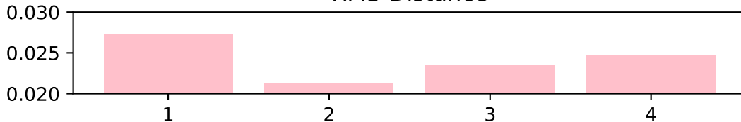
RMS-Distance
