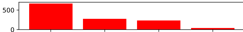
MFCC-Distance
