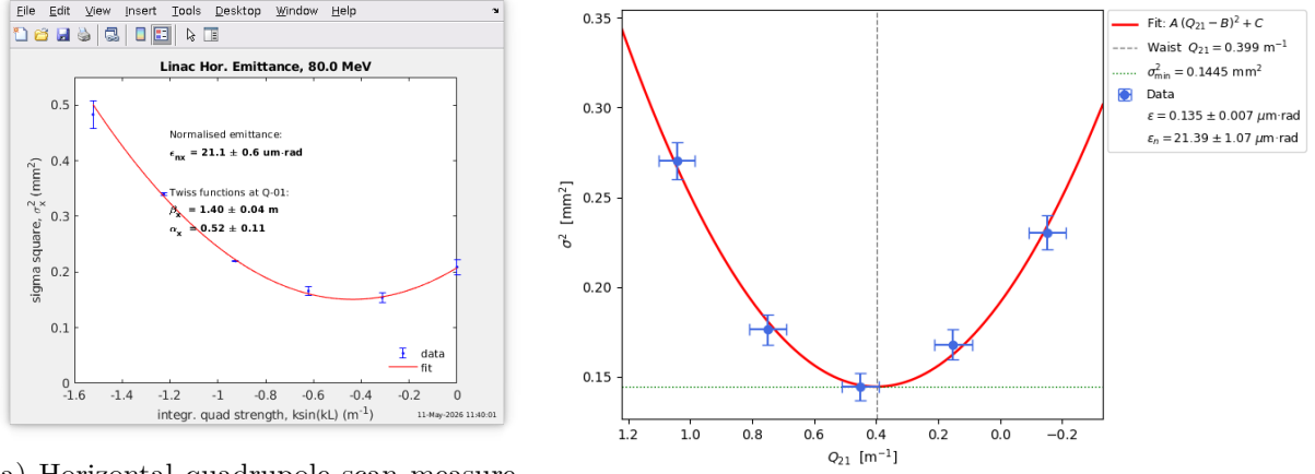
(a) Horizontal quadrupole scan measurements from the ALBA control room GUI.
