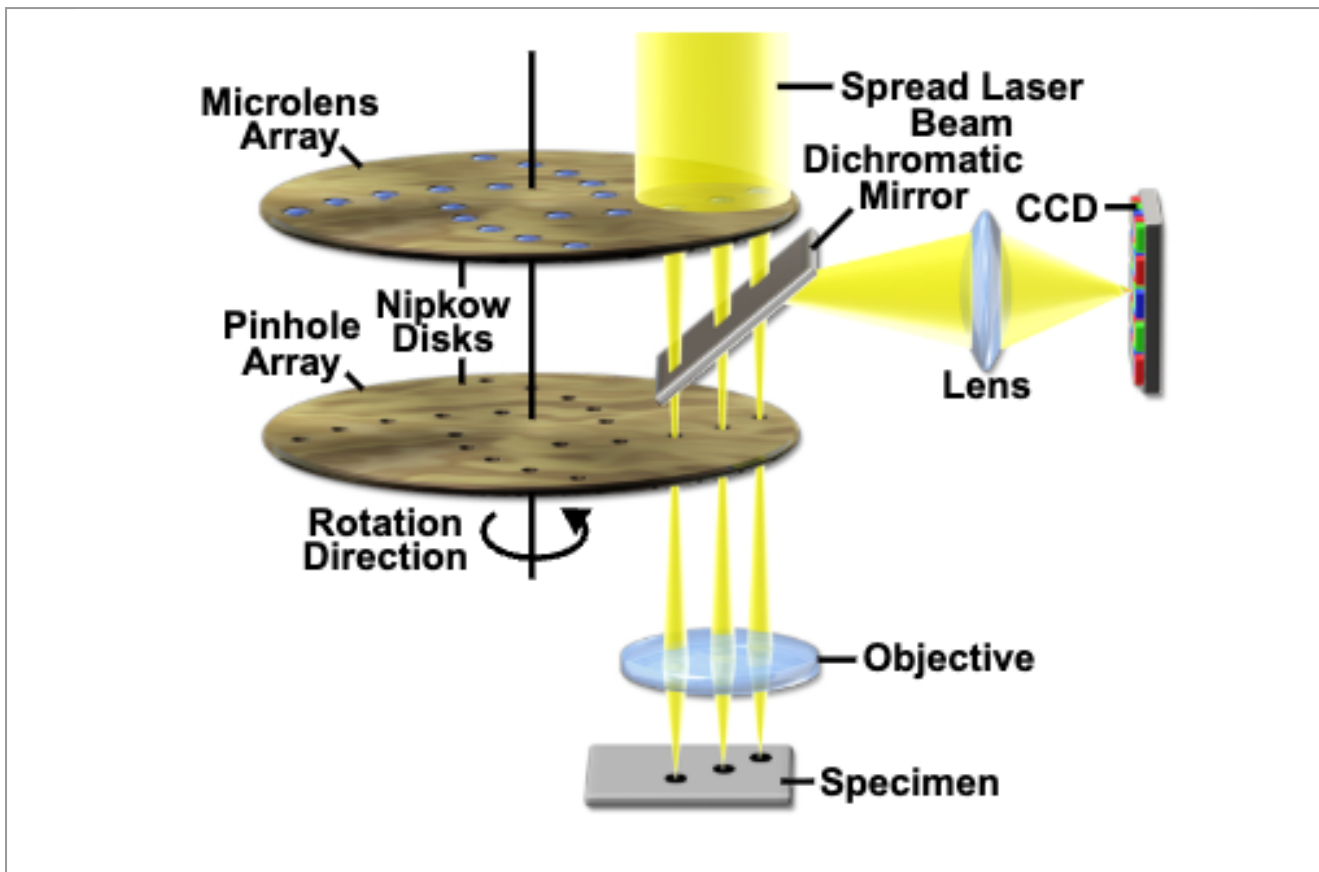
Figure 12. Nipkow disk configuration (From: MicroscopyU)
