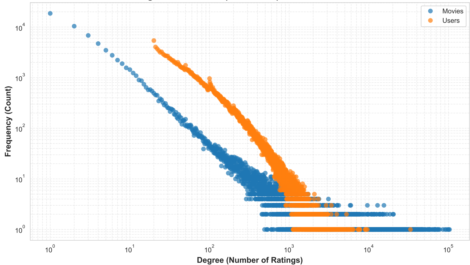
Degree Distribution (Power Law): Users and Movies
