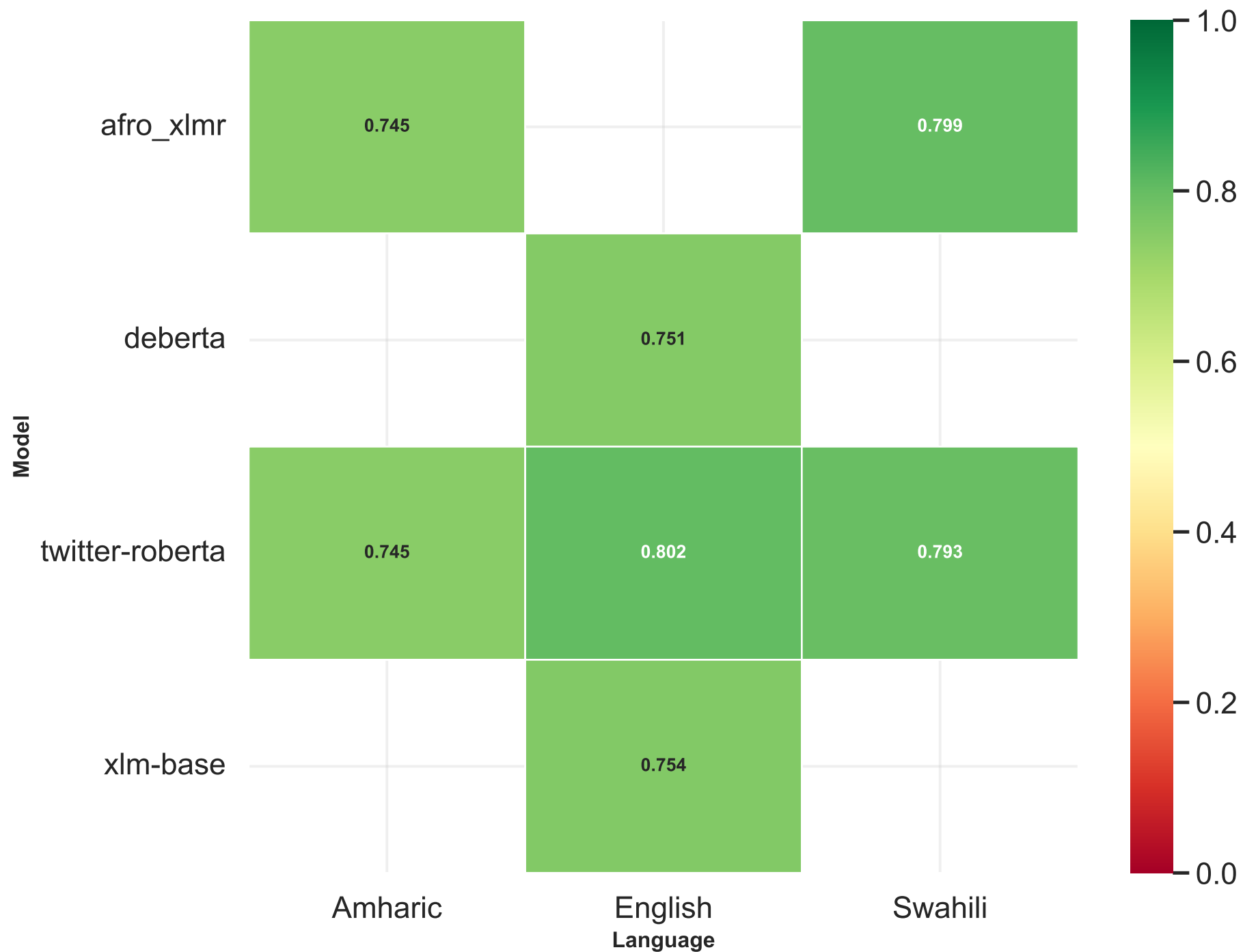
Subtask 1: Binary Polarization Detection Heatmap Analysis
