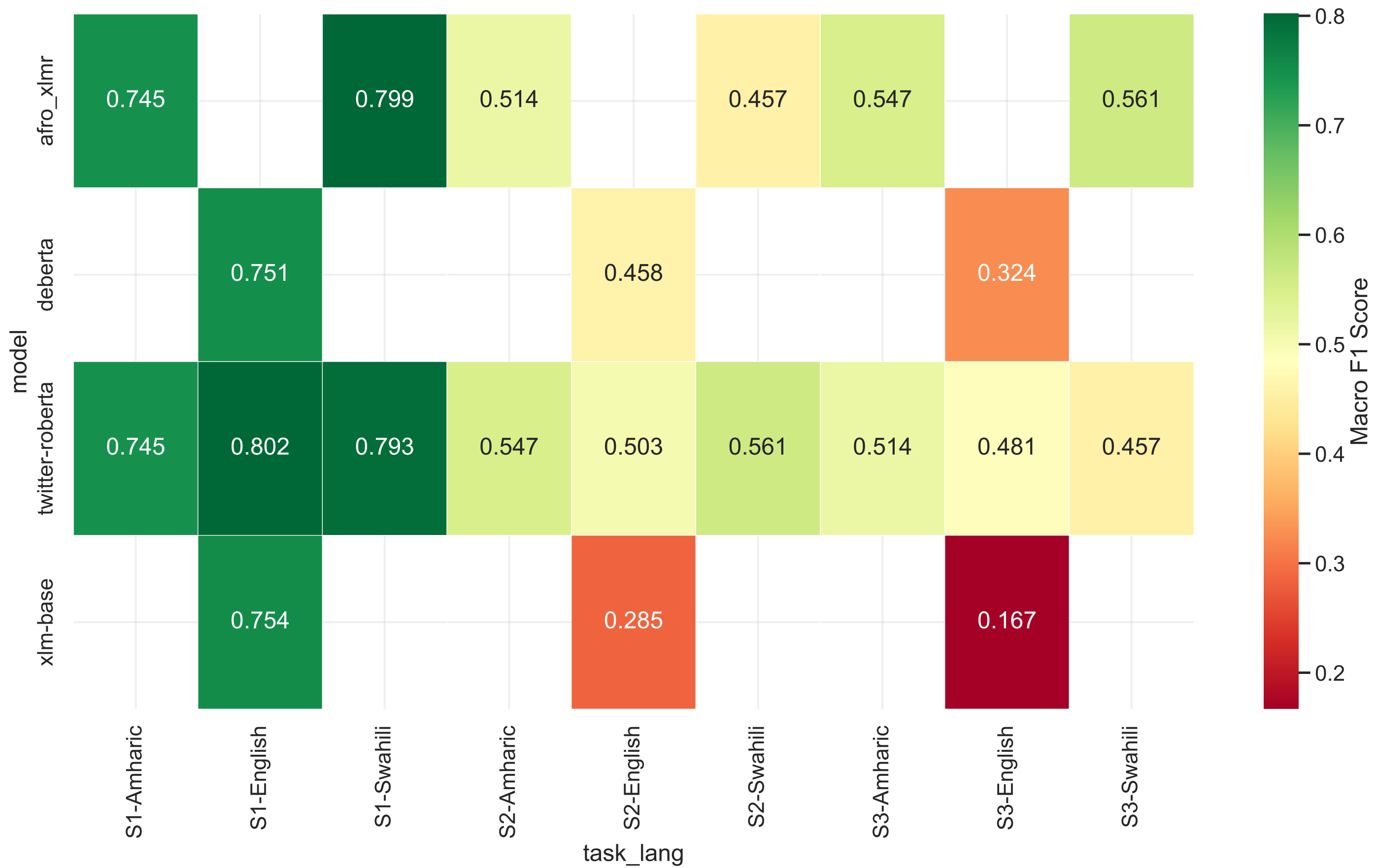
Global Performance Heatmap (All Subtasks)
