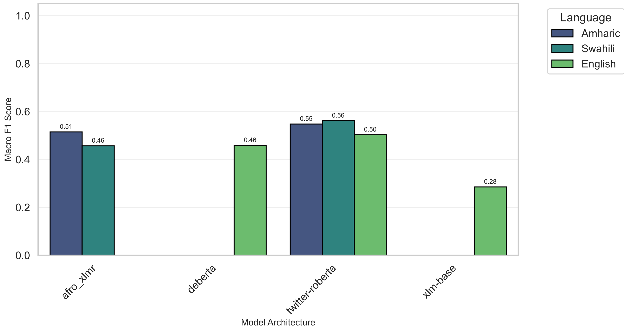
Multi-Label Classification - Model Performance
