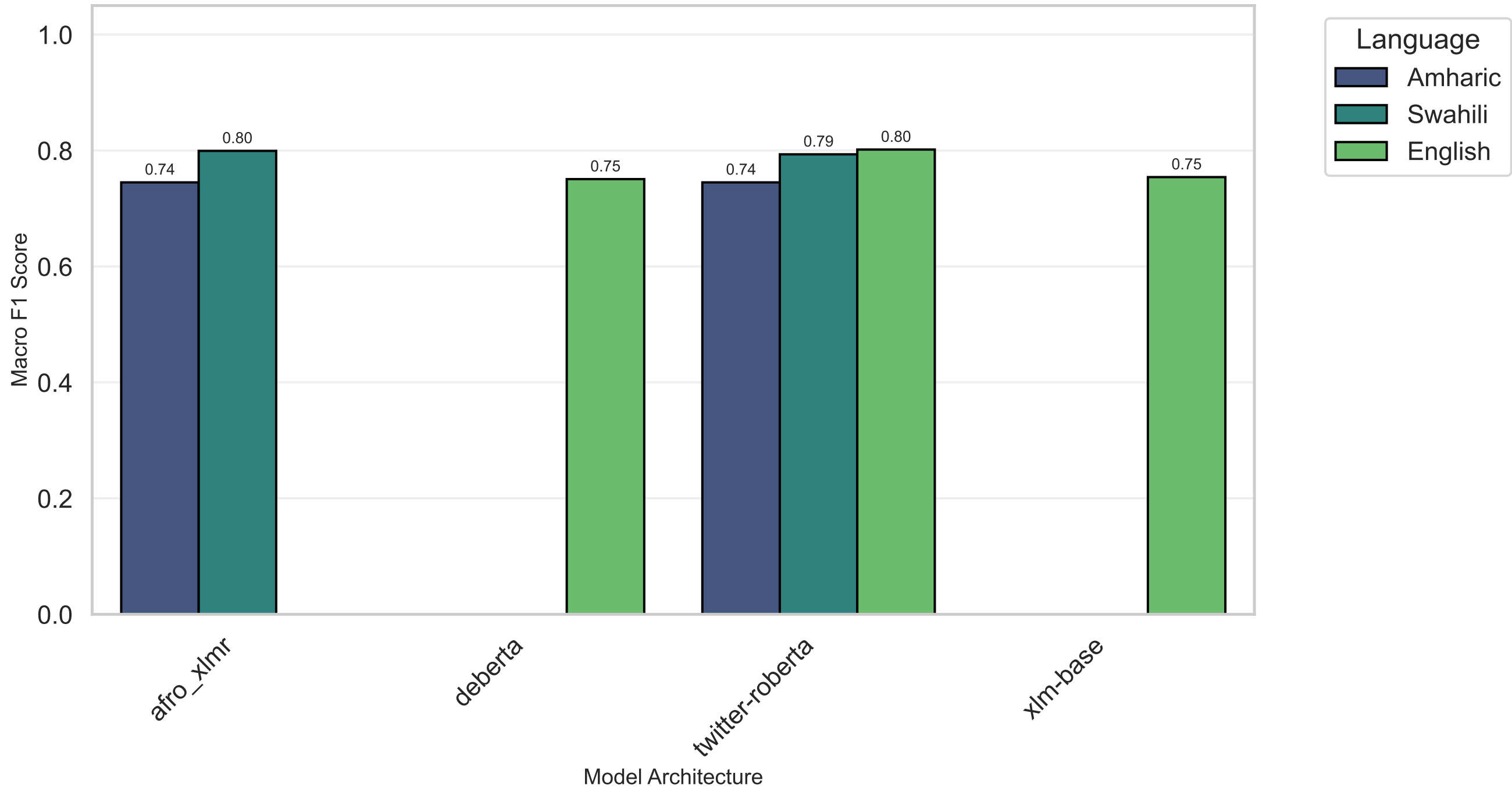
Binary Polarization - Model Performance
