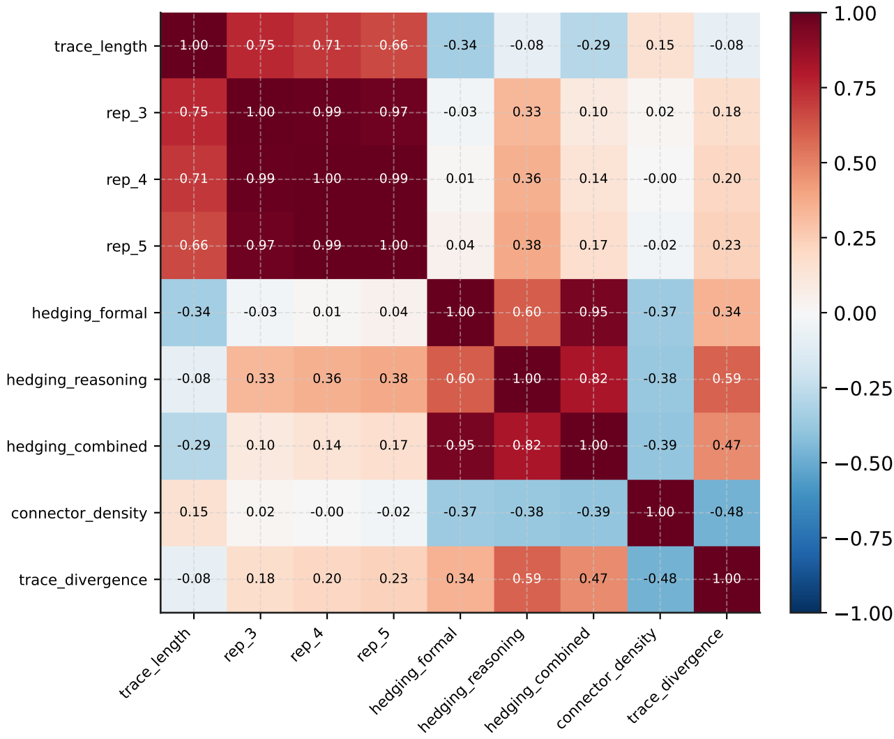
Qwen3-4B — feature Pearson r (pooled across that model's datasets)
