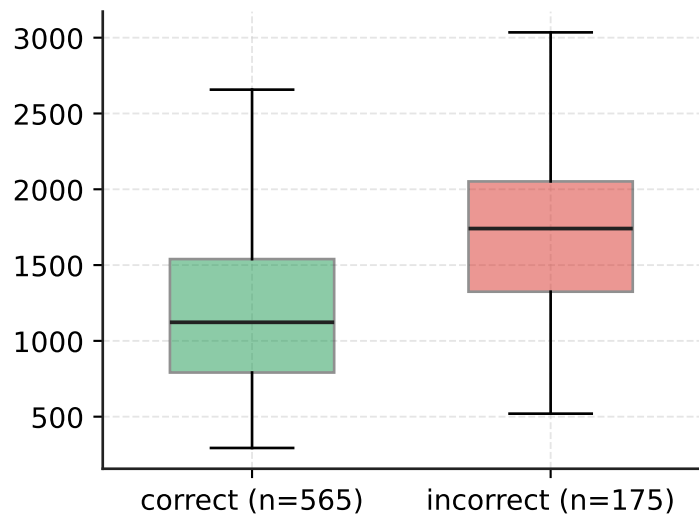
hedging_reasoning
