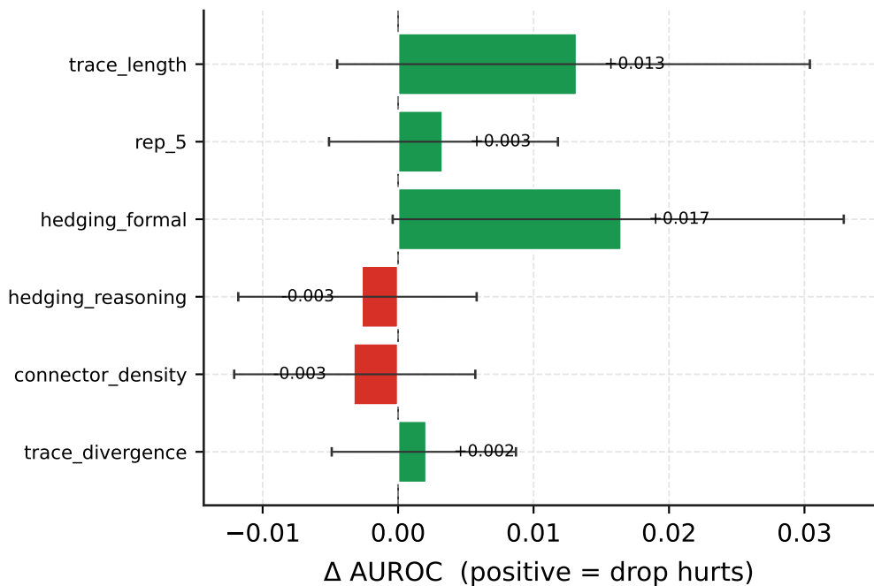
medqa (full AUROC = 0.667)
