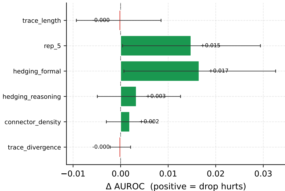
medqa (full AUROC = 0.780)
