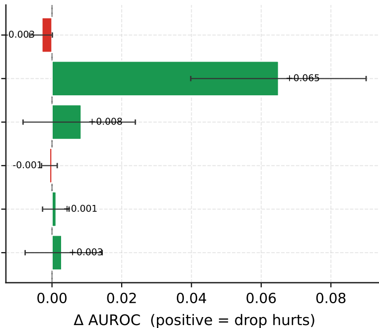
mmlu_pro (full AUROC = 0.817)
