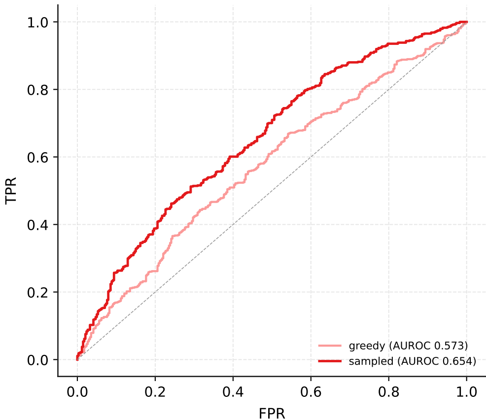
Llama-3.1-8B-Instruct (CoT) / medqa
