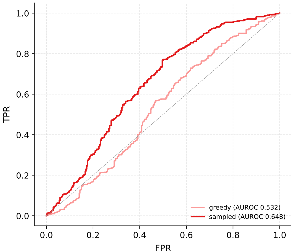
Llama-3.1-8B-Instruct (CoT) / trivia_qa
