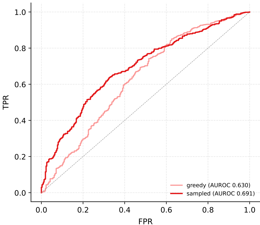
Qwen3-4B (thinking off, CoT) / mmlu_pro
