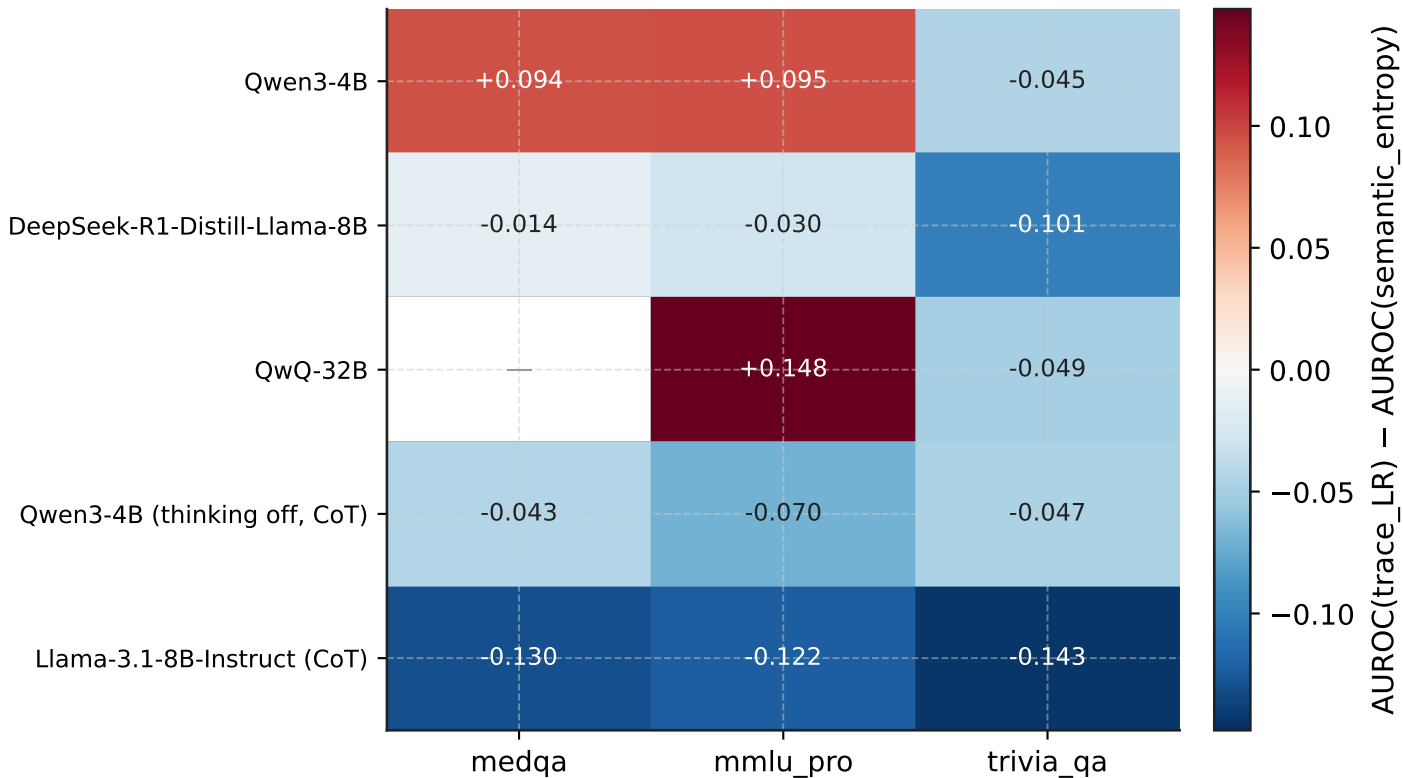
trace_LR – semantic_entropy (positive \Rightarrow trace_LR wins)
