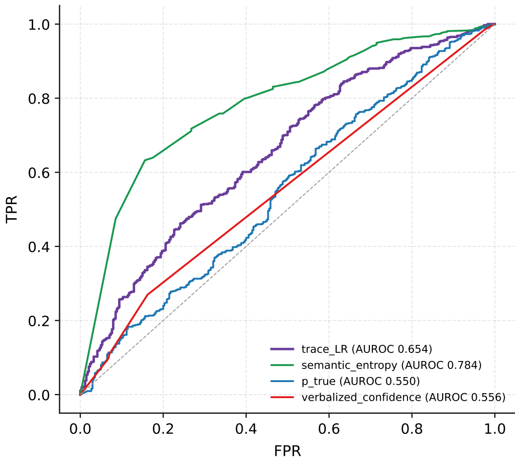
Llama-3.1-8B-Instruct (CoT) / medqa
