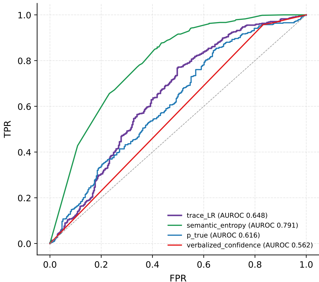
Llama-3.1-8B-Instruct (CoT) / trivia_qa
