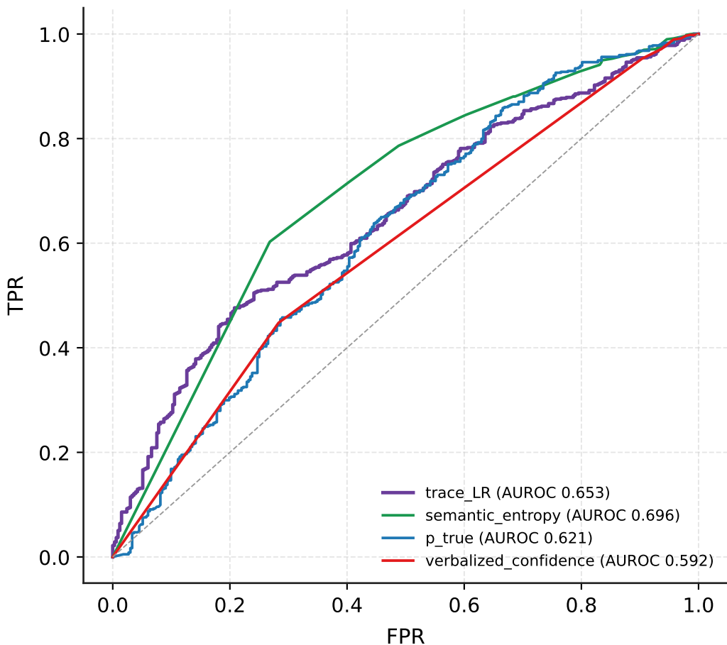
Qwen3-4B (thinking off, CoT) / medqa
