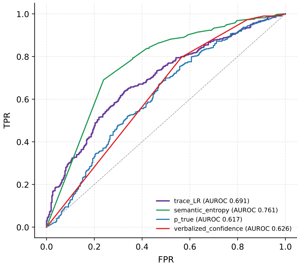
Qwen3-4B (thinking off, CoT) / mmlu_pro
