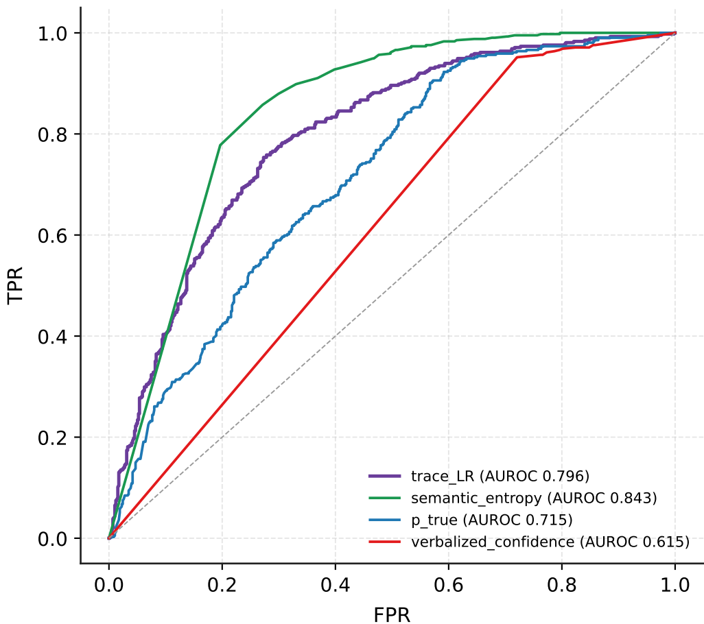
Qwen3-4B (thinking off, CoT) / trivia_qa
