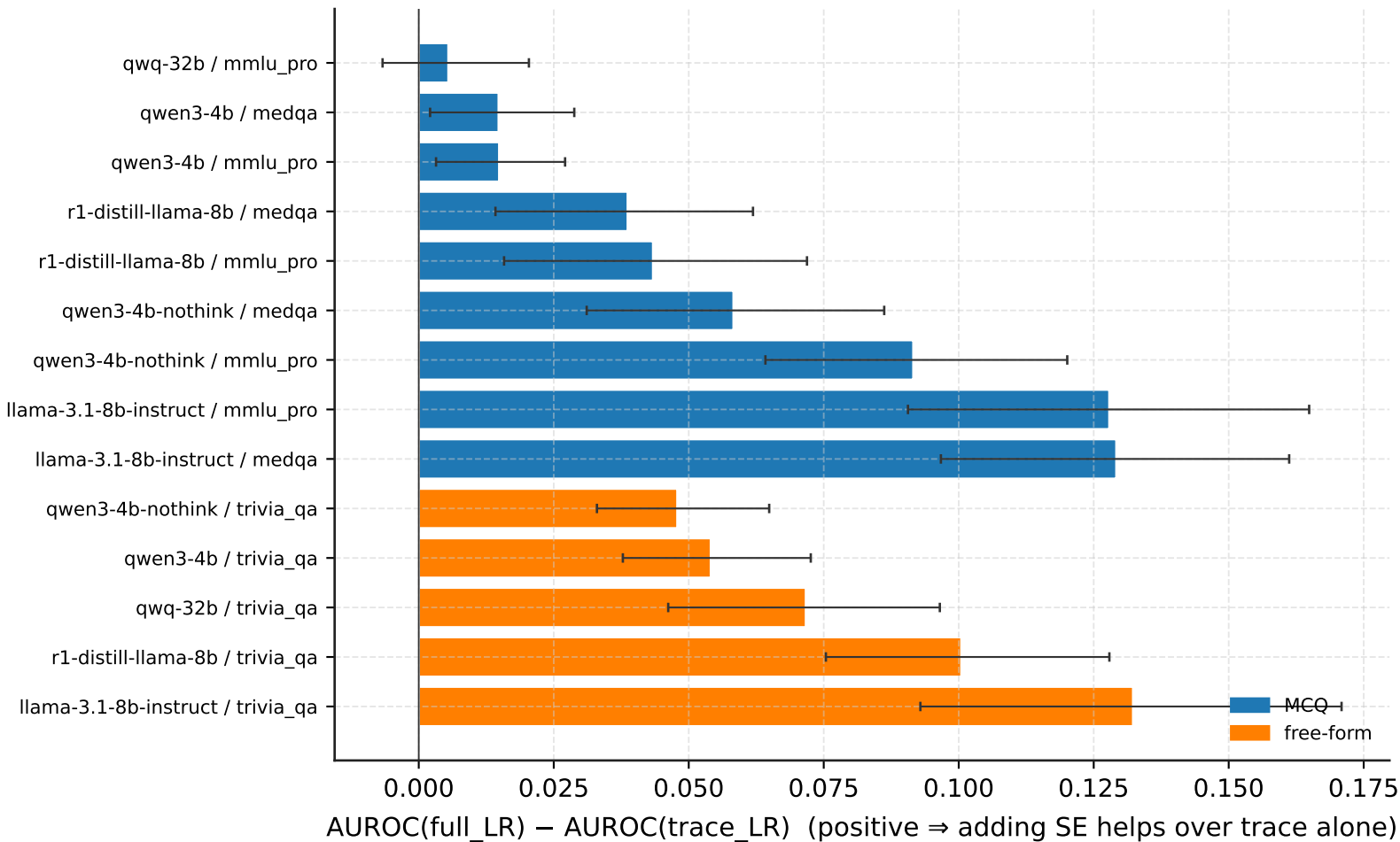
How much does adding semantic_entropy to trace_LR help, per cell?
