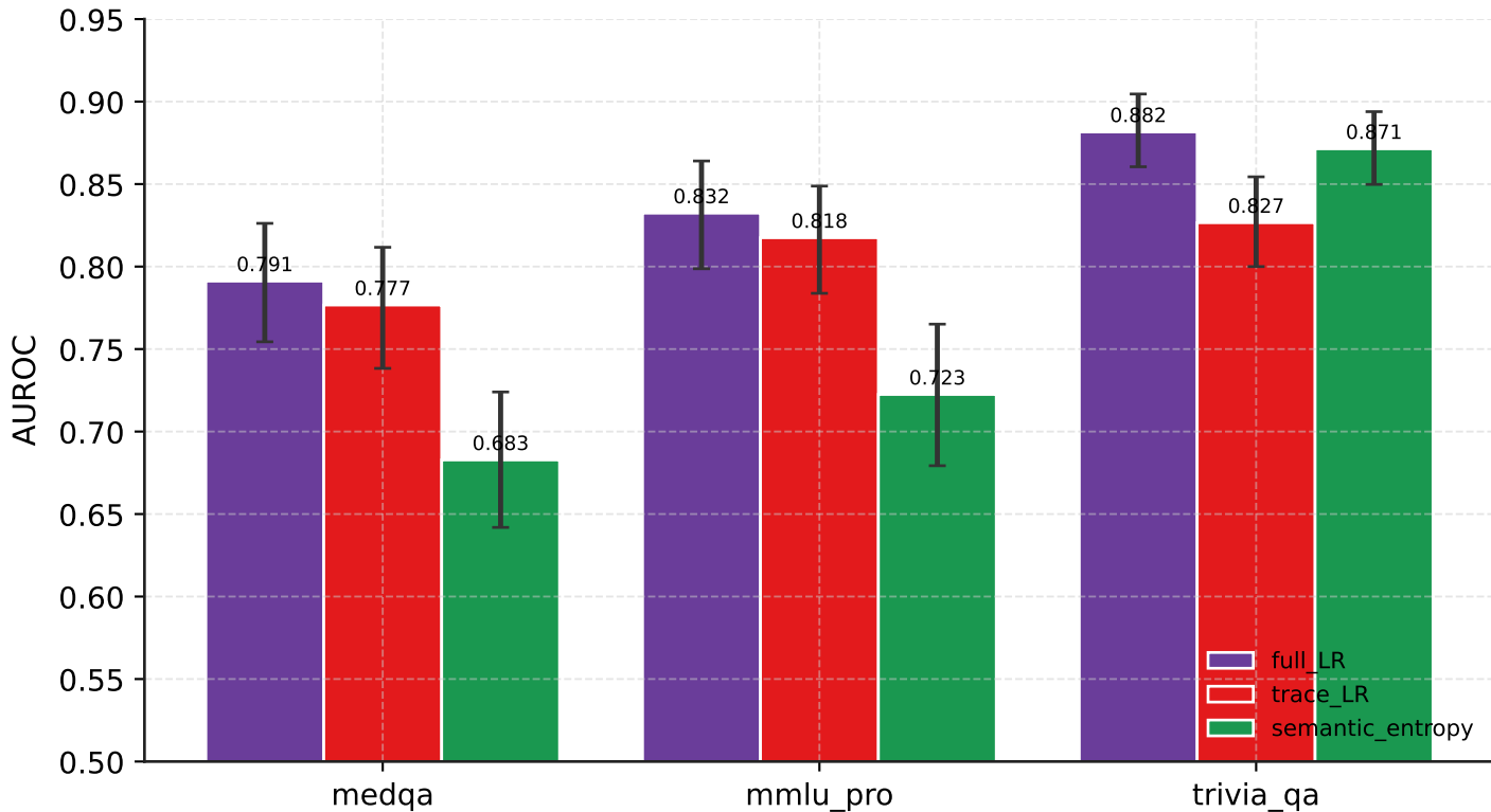
Qwen3-4B — full_LR vs trace_LR vs semantic_entropy (AUROC, 95 % bootstrap CI)
