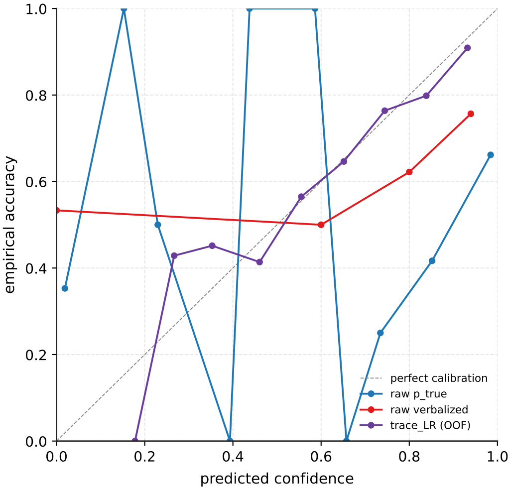
Llama-3.1-8B-Instruct (CoT) / medqa — reliability
