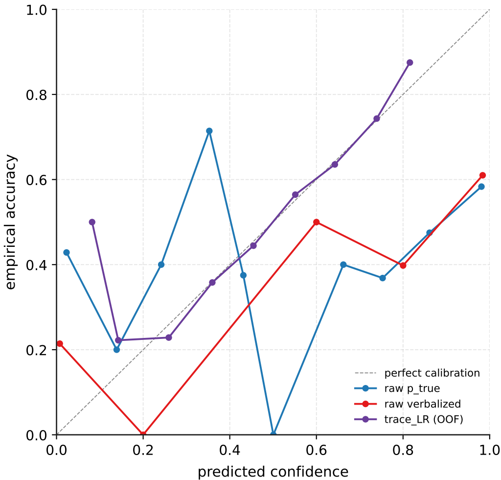
Llama-3.1-8B-Instruct (CoT) / mmlu_pro — reliability
