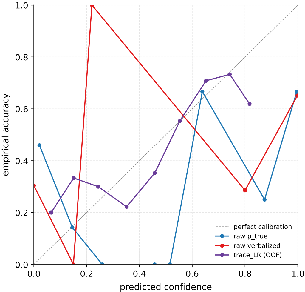
Llama-3.1-8B-Instruct (CoT) / trivia_qa — reliability
