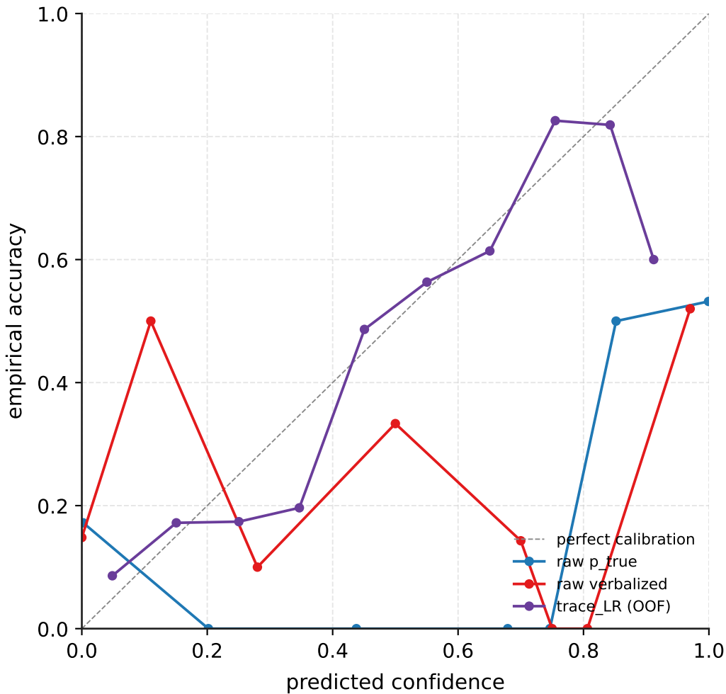
Qwen3-4B / trivia_qa — reliability
