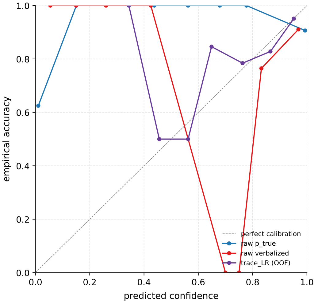
QwQ-32B / mmlu_pro — reliability
