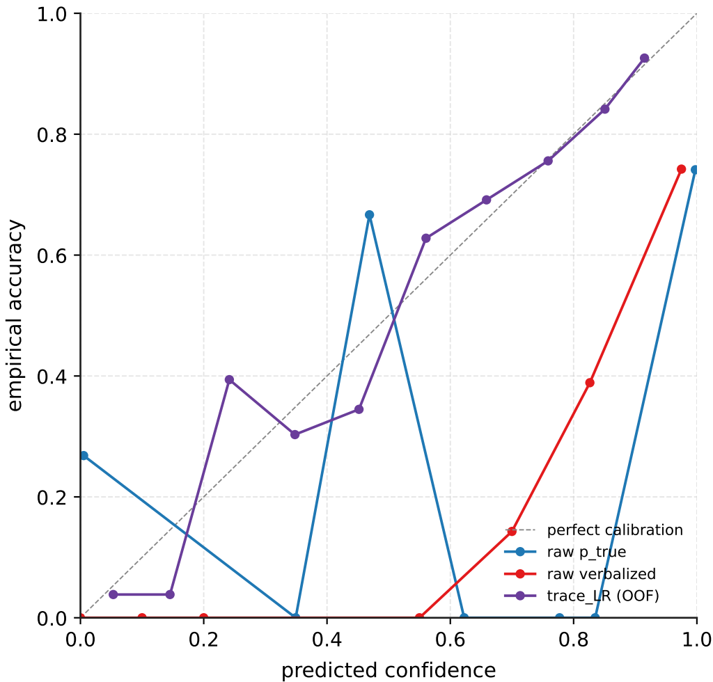
QwQ-32B / trivia_qa — reliability
