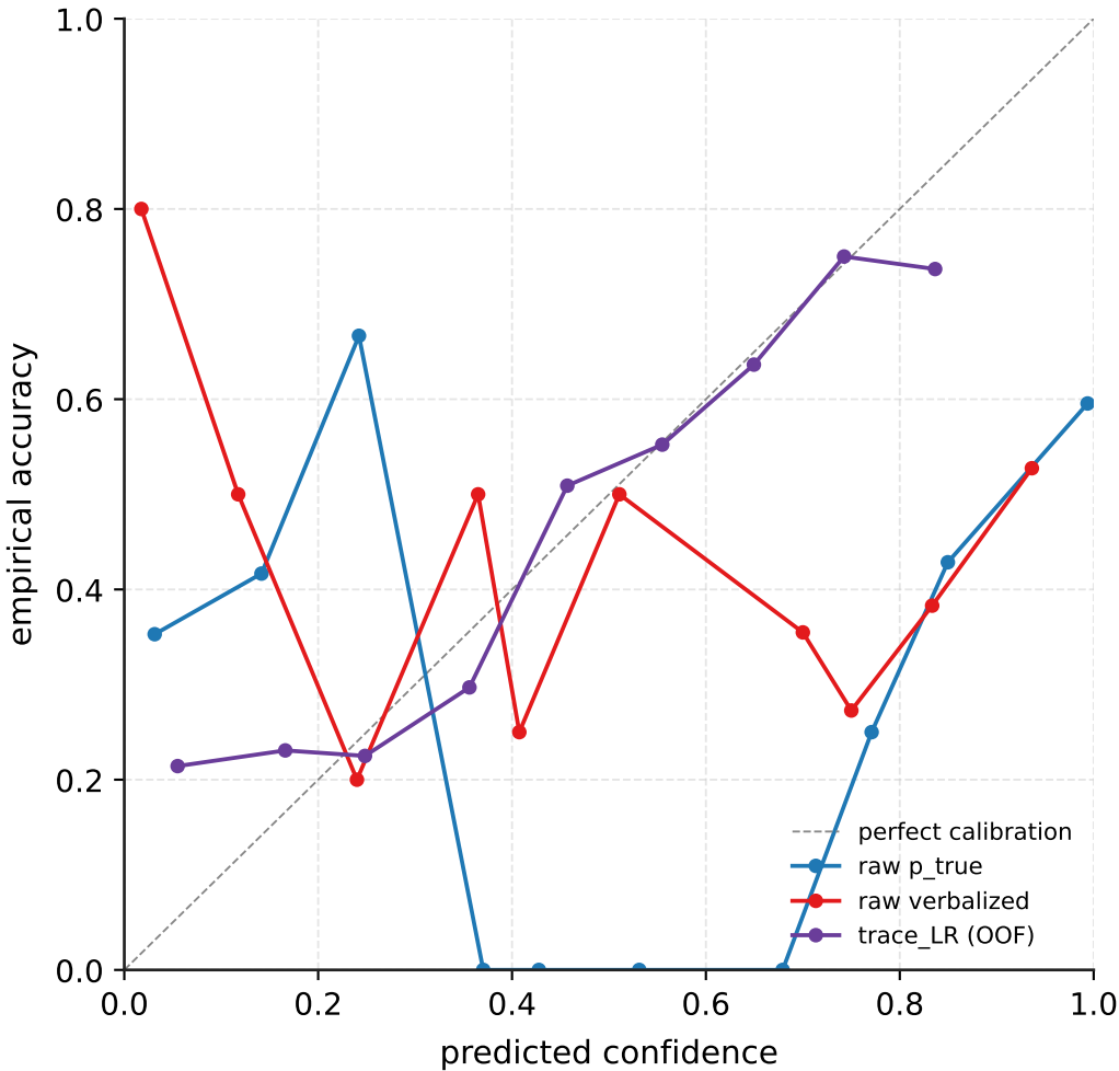
DeepSeek-R1-Distill-Llama-8B / mmlu_pro — reliability
