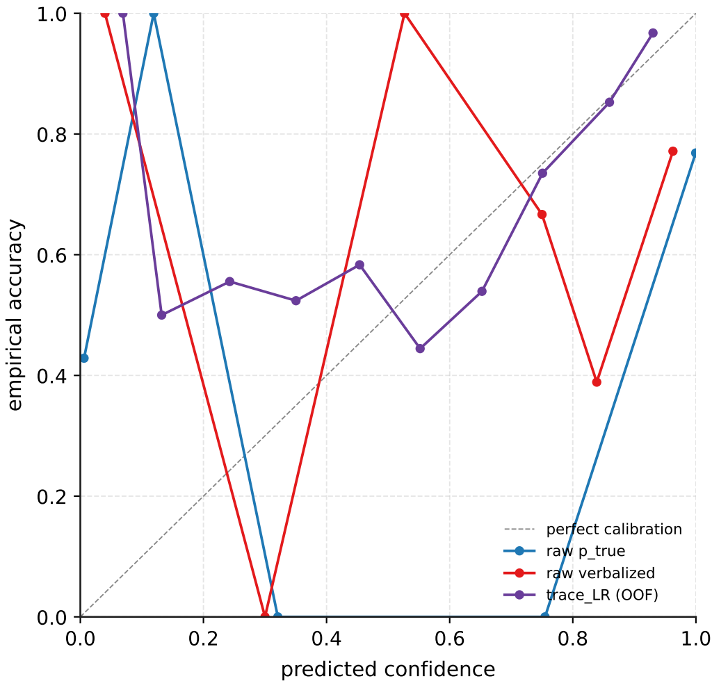
Qwen3-4B / medqa — reliability
