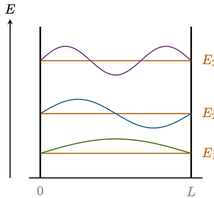
Figure 2. Infinite square well: energy levels E_n \propto n^2 (orange) and corresponding eigenfunctions \psi_1 , \psi_2 and \psi_3 (olive, blue and plum).
