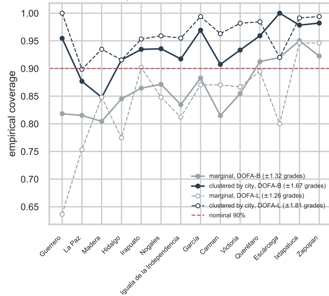
c Coverage holds only when cities are clustered
