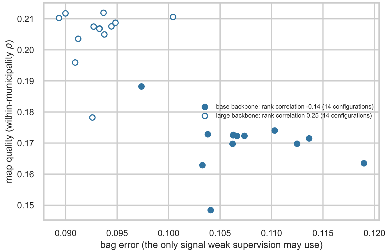
b Aggregate validation cannot see map quality
