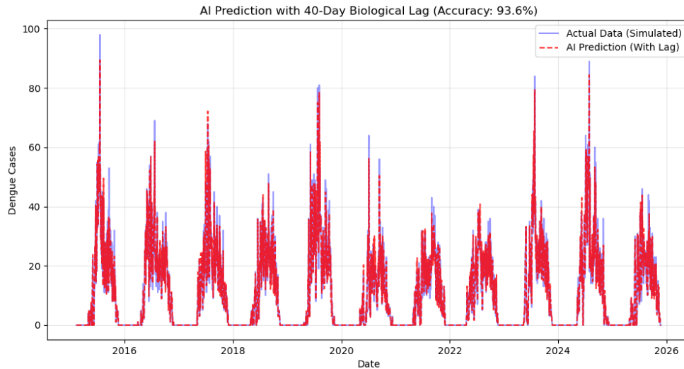
Figure 2: AI Prediction (Red) vs Actual Data (Blue). The AI follows the pattern very well.
