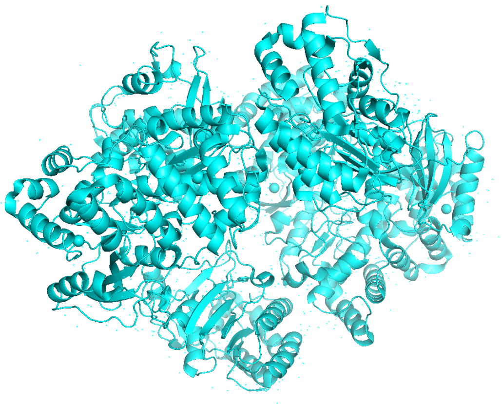
Figure 3: 3D Structure of the Dengue Virus NS5 Protein (PDB: 5ZQK). I generated this image using PyMOL.
