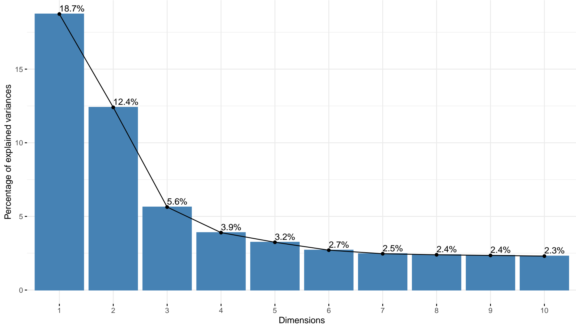
Scree plot
