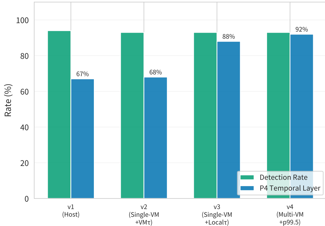
(b) Detection Rate & Temporal Layer
