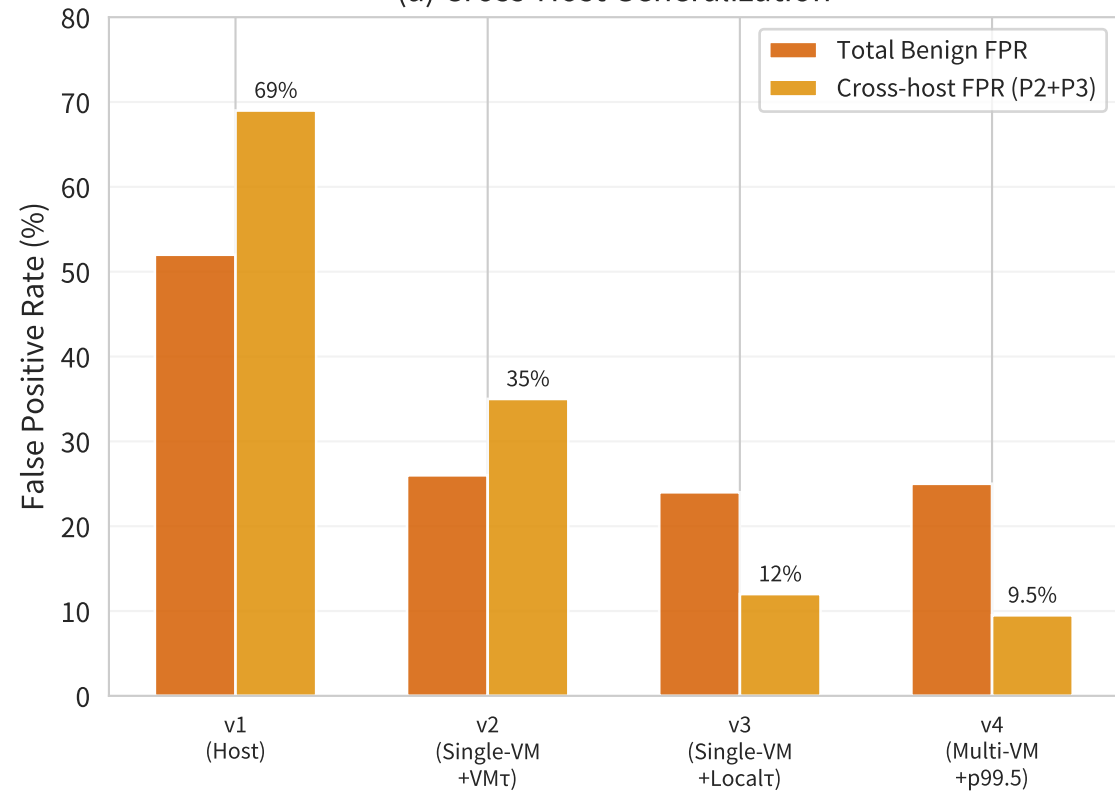
(a) Cross-Host Generalization
