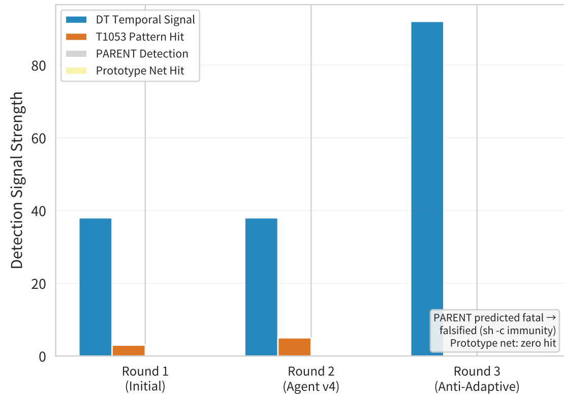
(a) Adversarial Round Evolution
