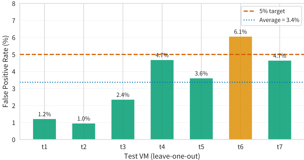
Cross-Host Generalization on 7 Unseen VMs
