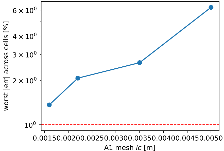
(a) A1 current disc: envelope
