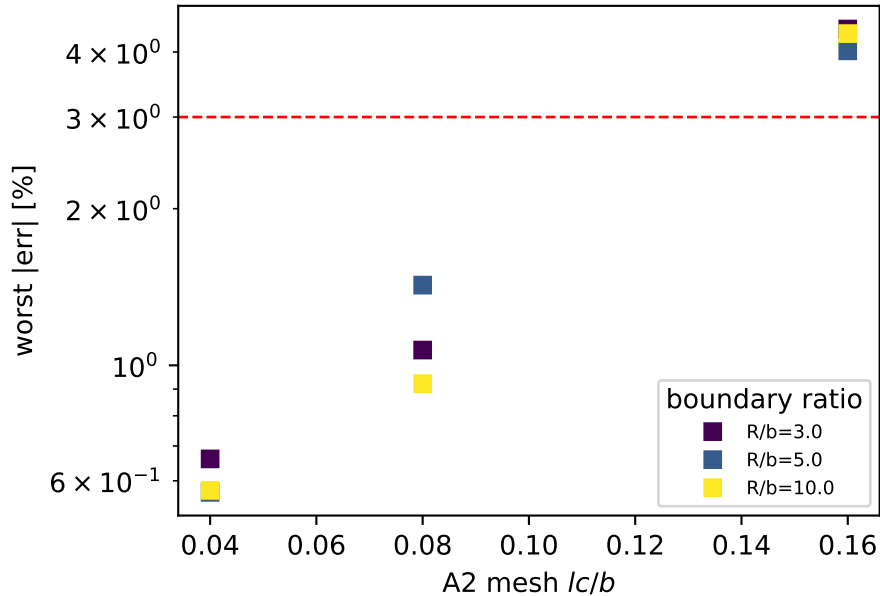
(b) A2 cylinder: covered zone R/b \geq 3
