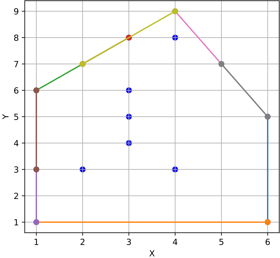
Scatter Plot of ConvexHull- by: Deniz DAHMAN, PhD
