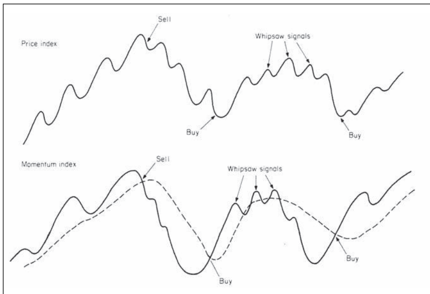
Figura 13.21 MA Crossovers
