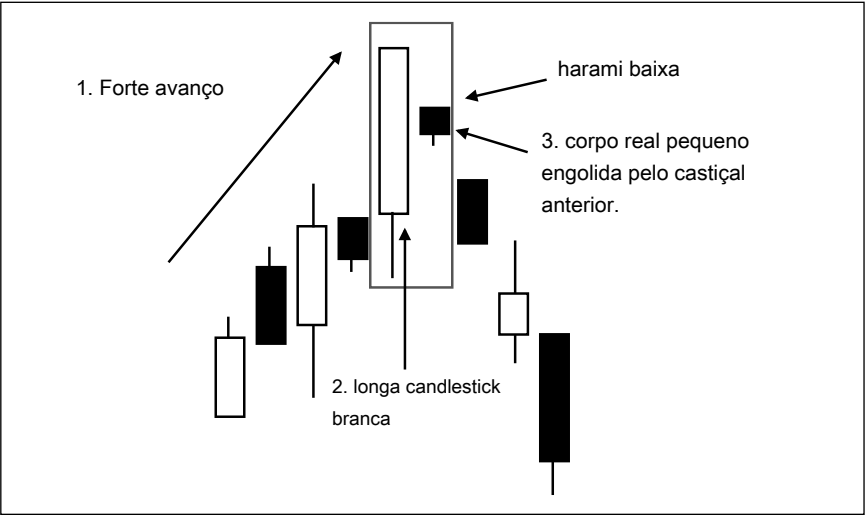
Figura 16.29 bearish Harami
