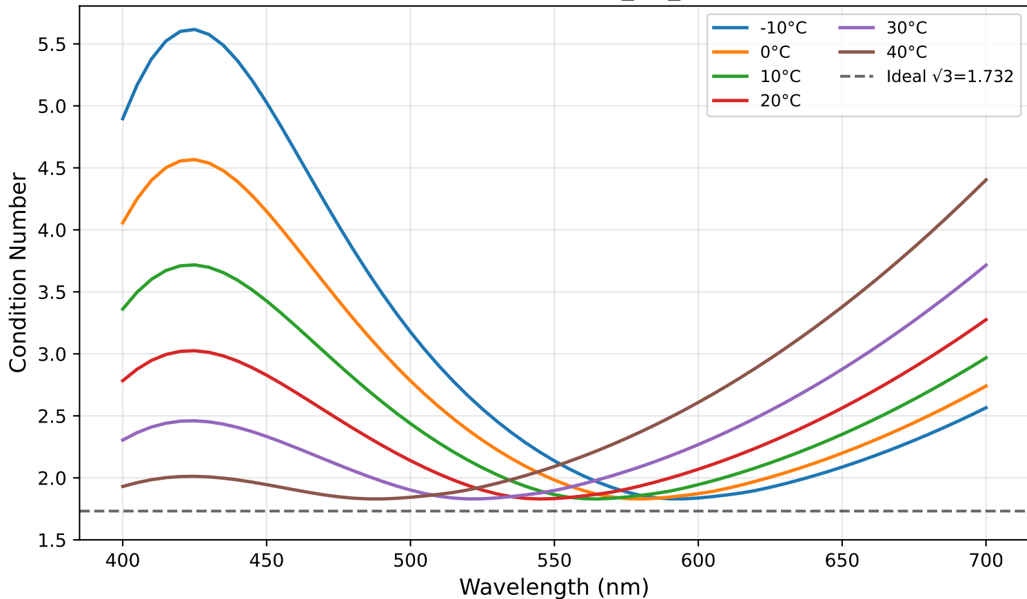
CN vs Wavelength — A_CN_4meas
