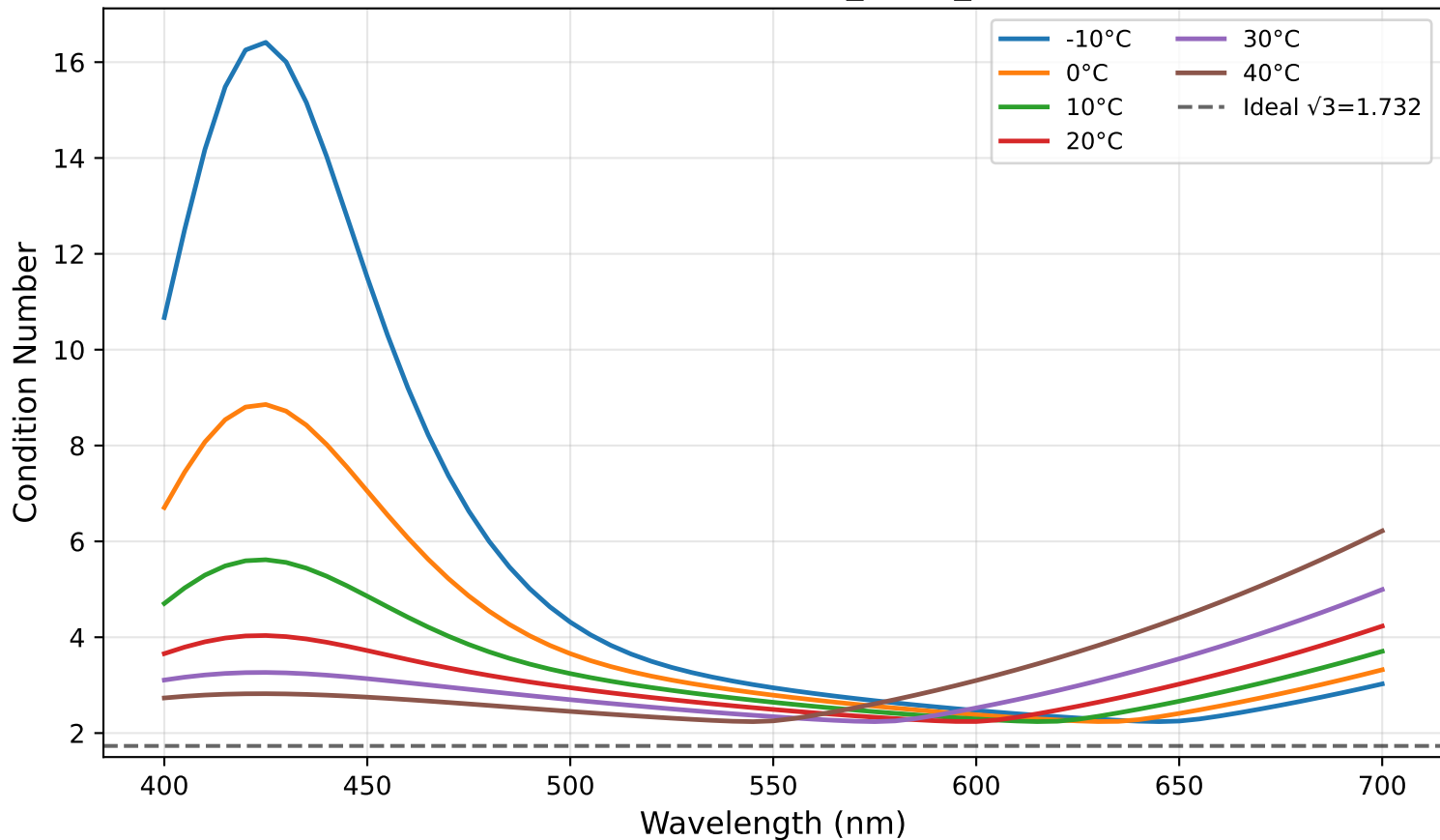
CN vs Wavelength — B_BCPN_4meas
