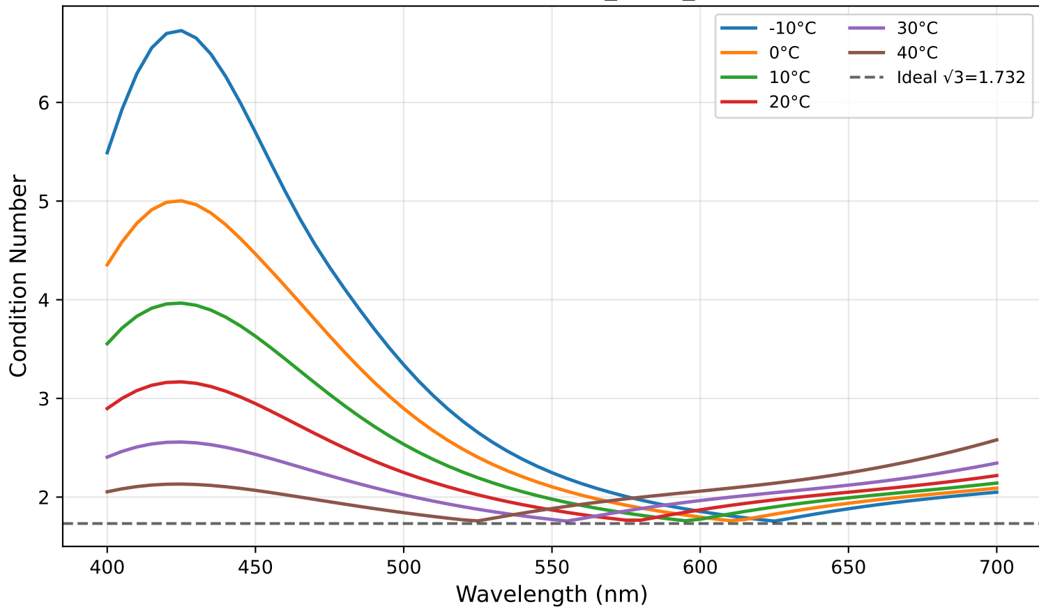
CN vs Wavelength — B_BCPN_6meas
