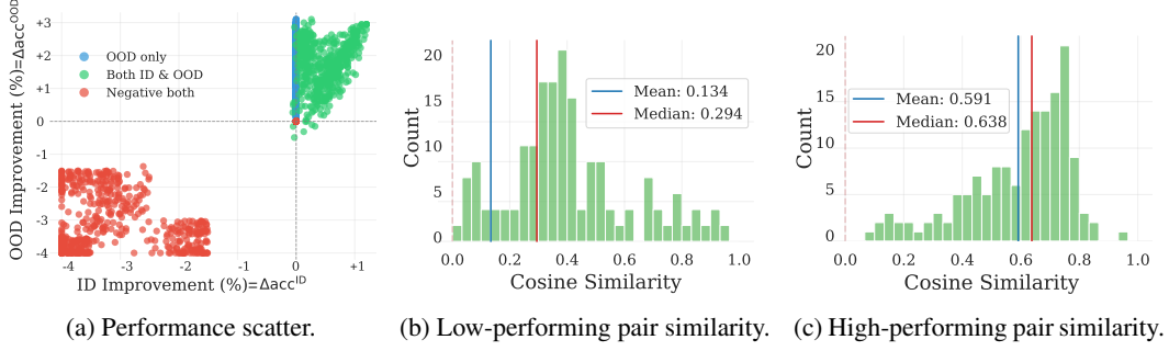
Figure 2: Performance and alignment analysis of Model Stock on 2415 pairwise combinations of CLIP ViT-B/32 models fine-tuned on ImageNet. (a) Scatter plot of ID vs. OOD performance relative to the better constituent model. (b) and (c): Layer-wise cosine similarity for low-performing and high-performing, respectively. Stronger alignment coincides with consistent gains, highlighting that alignment can serve as a key predictor of merging success.
