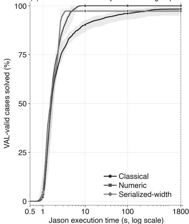
(b) Time-to-valid-trace by benchmark group
