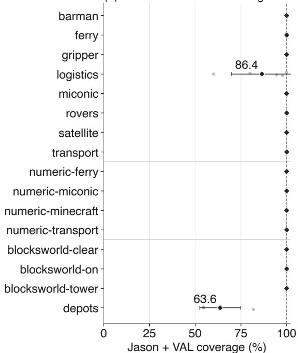
(a) Five-seed held-out coverage
