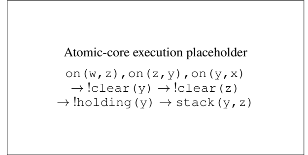
Figure 3: Execution of the selected atomic core in Blocks World. From \text{on}(w, z), \text{on}(z, y), \text{on}(y, x) , the goal !\text{on}(y, z) calls !\text{clear}(y) . The same clear/1 module recurs on z , decreasing the certified obstruction count before holding/1 and the direct stack(y, z) producer complete the goal. The selected rules contain variables rather than these illustrative object names.
