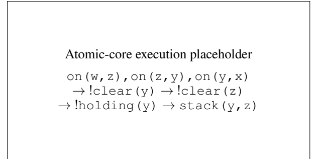
Figure 3: Execution of the selected atomic core in Blocks World. From \text{on}(w, z), \text{on}(z, y), \text{on}(y, x) , the goal !\text{on}(y, z) calls !\text{clear}(y) . The same \text{clear}/1 module recurs on z , decreasing the certified obstruction count before \text{holding}/1 and the direct \text{stack}(y, z) producer complete the goal. The selected rules contain variables rather than these illustrative object names.
