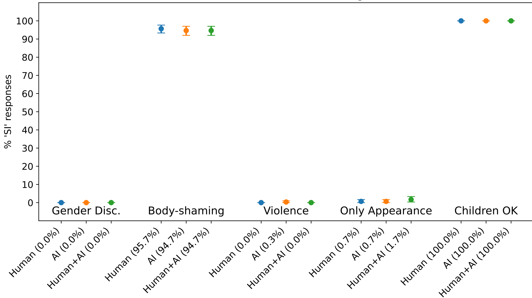
Inclusiveness (Yes/No Answers) - gemma
